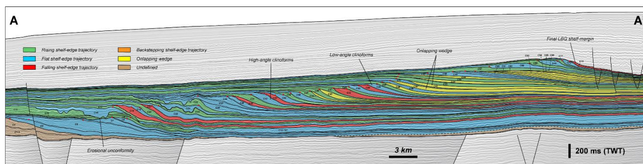
Figure 2: Example of seismic profile from the Investigator Depocentre (see location on Fig. 3) showing the 73 interpreted clinothems with the corresponding types of shelf-margin architecture based on trajectory analysis. Data courtesy of TGS.
