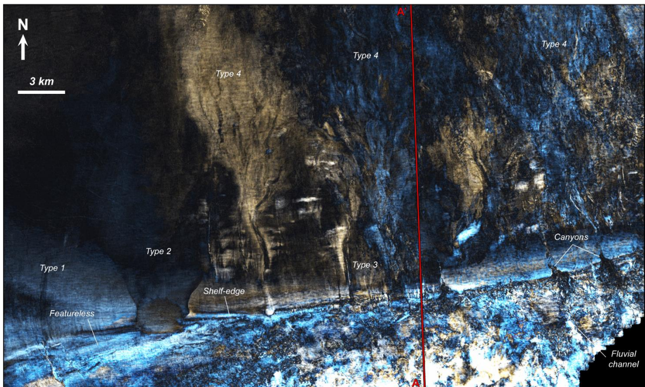
Figure 3: Example of colour-blended (RGB) spectral decomposition map (at 15, 35 and 55 Hz) of one horizon from the clinothem C28 (see Fig. 2) showing interpreted seismic geomorphologies at the shelf-edge (i.e. shallow-marine processes) and the deep-water system types. Data courtesy of TGS.
