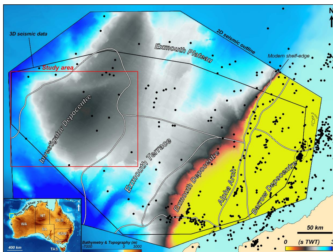
Figure 1: Location map of the study area within the Northern Carnarvon Basin (North West Shelf, Australia). The map corresponds to the seafloor horizon interpreted on regional 2D seismic data. The geological provinces indicated on this map correspond to the Lower Barrow Group depocentres interpreted by Paumard et al. (2018).
